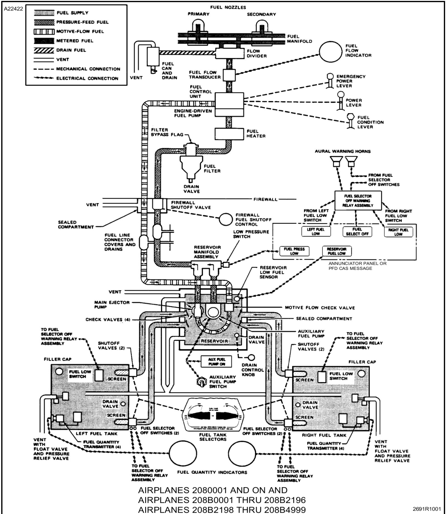
Figure 1 : Sheet 2 : Fuel System Schematic
